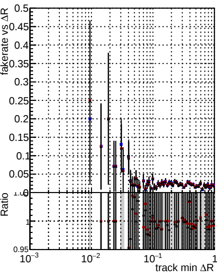
Fake rate vs \Delta R(\text{track, jet}) Legend: DQM_XiMinus_original_lowpt DQM_XiMinus_newbranch_lowpt_pLess DQM_XiMinus_newbranch_lowpt_pLessMVACand
