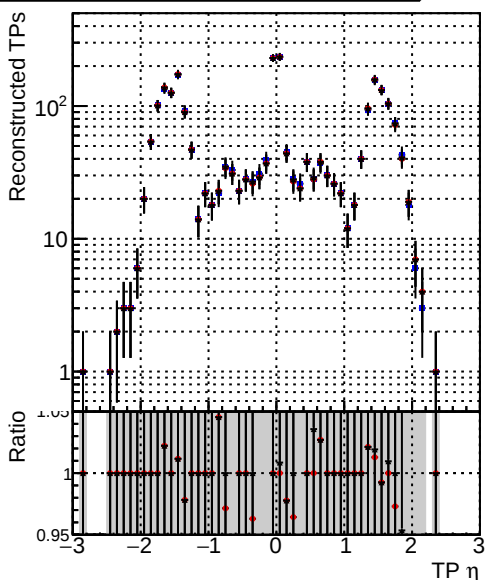
—•— DQM_XiMinus_original_lowpt —•— DQM_XiMinus_newbranch_lowpt_pLess —•— DQM_XiMinus_newbranch_lowpt_pLessMVACand
