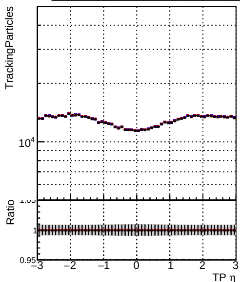
Legend: DQM_XiMinus_original_lowpt (blue line with dots) DQM_XiMinus_newbranch_lowpt_pLess (red line with dots) DQM_XiMinus_newbranch_lowpt_pLessMVACand (black line with dots)
