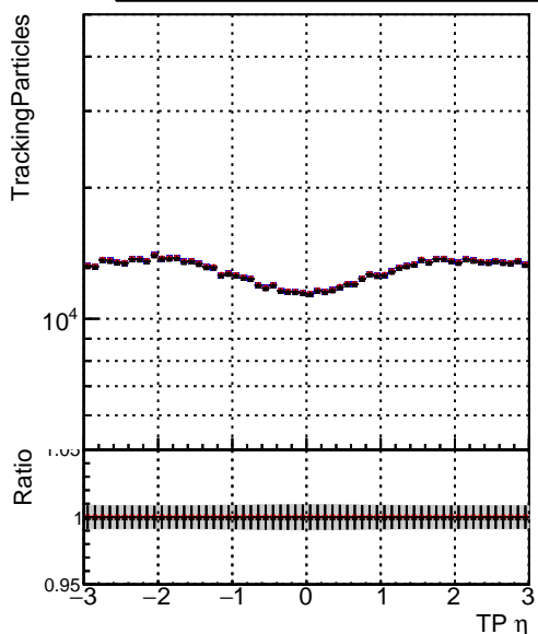
Legend: DQM_XiMinus_original_lowpt DQM_XiMinus_newbranch_lowpt_pLess DQM_XiMinus_newbranch_lowpt_pLessMVACand
