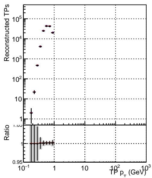
Legend: DQM_XiMinus_original_lowpt DQM_XiMinus_newbranch_lowpt_pLess DQM_XiMinus_newbranch_lowpt_pLessMVACand
