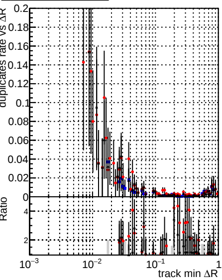
Legend: DQM_XiMinus_original_lowpt (black line with blue dots), DQM_XiMinus_newbranch_lowpt_pLess (red line with red dots), DQM_XiMinus_newbranch_lowpt_pLessMVACand (black line with black dots)
