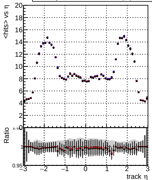
— DQM_XiMinus_original_lowpt — DQM_XiMinus_newbranch_lowpt_pLess — DQM_XiMinus_newbranch_lowpt_pLessMVACand
