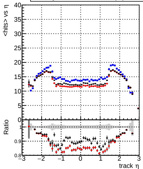
mean hits — DQM_XiMinus_original_lowpt — DQM_XiMinus_newbranch_lowpt_pLess — DQM_XiMinus_newbranch_lowpt_pLessMVACand
