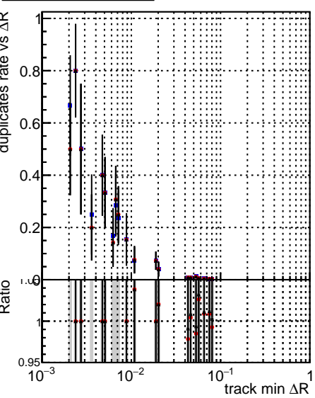
■ DQM_XiMinus_original_lowpt ● DQM_XiMinus_newbranch_lowpt_pLess ▲ DQM_XiMinus_newbranch_lowpt_pLessMVACand
