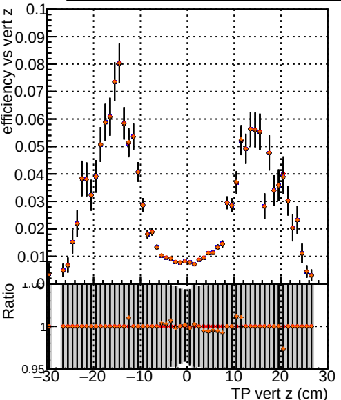
Efficiency vs vertpos DOM_XiMinus_original_lowpt DOM_XiMinus_newbranch_lowpt DOM_XiMinus_original_lowpt_pLess DOM_XiMinus_newbranch_lowpt_pLess
