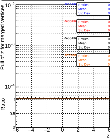
RecoAllAssoc2GenMatchedMerged_PullZ
