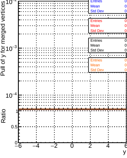
RecoAllAssoc2GenMatchedMerged_PullY
