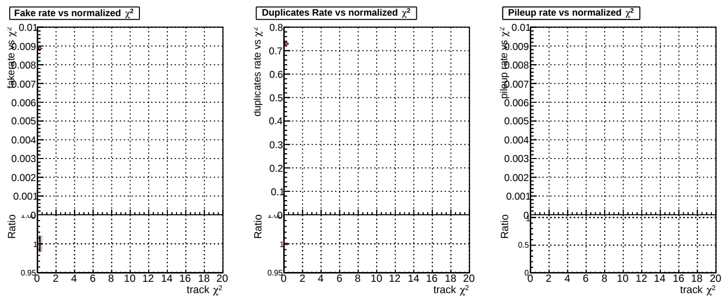
Fake rate vs. DOM x minus original lowpt DOM x minus devtoand lowpt DOM x minus devtoand lowpt pless DOM x minus newbranch lowpt pless
