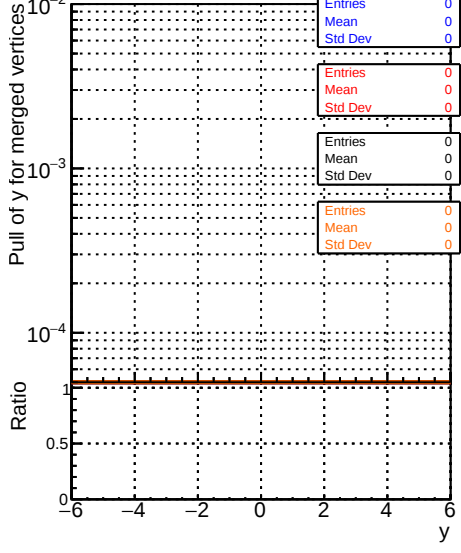
RecoAllAssoc2GenMatchedMerged_PullY
