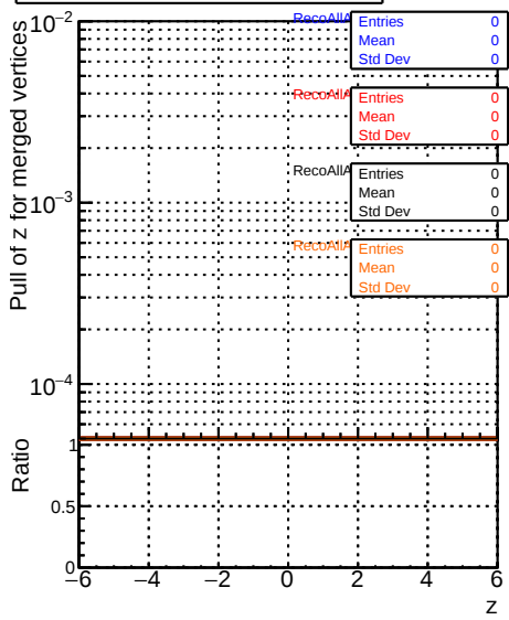
RecoAllAssoc2GenMatchedMerged_PullZ
