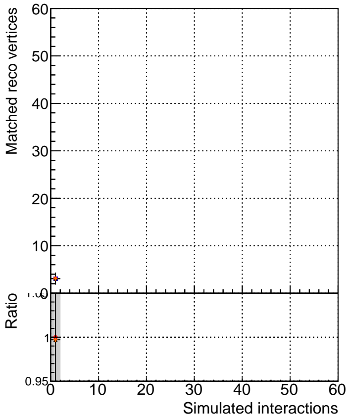
MatchedRecoVtx_vs_GenVtx
