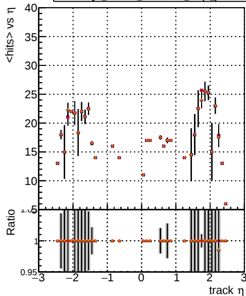
Legend: Blue line: DQM_XiMinus_original_lowpt Red line: DQM_XiMinus_newbranch_lowpt Black line: DQM_XiMinus_original_lowpt_pLess Orange line: DQM_XiMinus_newbranch_lowpt_pLess mean hit
