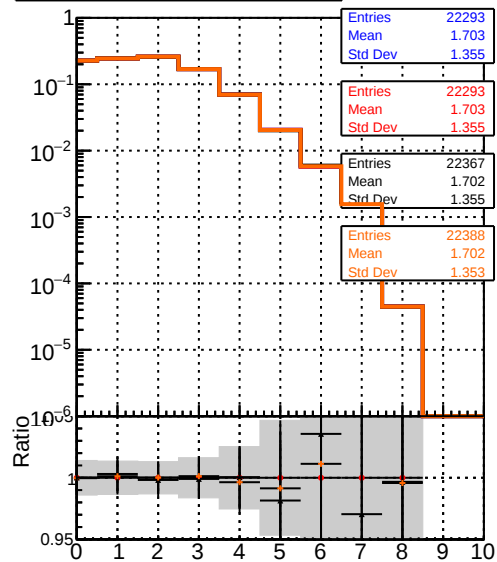
mean hits vs \eta DQM_XiMinus_original_lowpt DQM_XiMinus_newbranch_lowpt DQM_XiMinus_original_lowpt_pLess DQM_XiMinus_newbranch_lowpt_pLess
