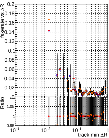
Fake rate vs \Delta R (track, jet) Legend: DOM X Minus original lowpt DOM X Minus newbranch lowpt DOM X Minus original lowpt pLess DOM X Minus newbranch lowpt pLess
