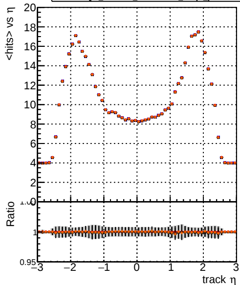
mean hits DQM_XiMinus_original_lowpt DQM_XiMinus_newbranch_lowpt DQM_XiMinus_original_lowpt_pLess DQM_XiMinus_newbranch_lowpt_pLess
