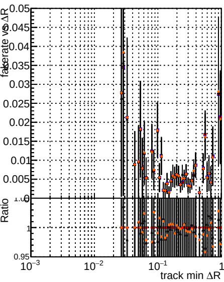
Fake rate vs ΔR(track, jet) Legend: DOM (black line) XiMinus (blue line) original lowpt (red line) newbranch lowpt pLess (orange line)
