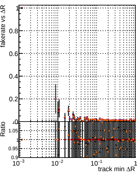
Fake rate vs ΔR(track, jet) for different models and pT thresholds Legend: DOM XiMinus original lowpt DOM XiMinus newbranch lowpt DOM XiMinus original lowpt pLess DOM XiMinus newbranch lowpt pLess
