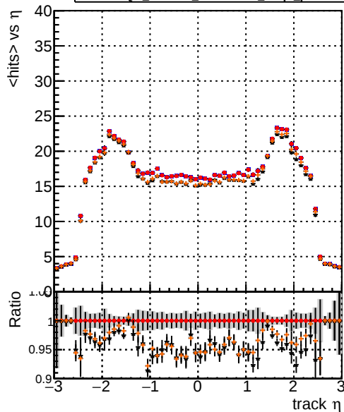
Legend: DQM_XiMinus_original_lowpt (blue line), DQM_XiMinus_newbranch_lowpt (red line), DQM_XiMinus_original_lowpt_pLess (black line), DQM_XiMinus_newbranch_lowpt_pLess (orange line) mean hits vs \eta
