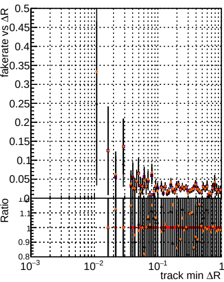
Fake rate vs \Delta R(\text{track, jet}) Legend: DOM (black line) XiMinus (blue line) original lowpt (red line) newbranch lowpt (orange line)
