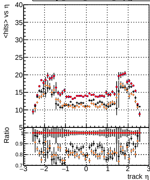
Legend: — DQM_XiMinus_original_lowpt (blue line) — DQM_XiMinus_newbranch_lowpt (red line) — DQM_XiMinus_original_lowpt_pLess (black line) — DQM_XiMinus_newbranch_lowpt_pLess (orange line) mean hits
