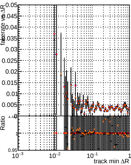
Fake rate vs \Delta R(\text{track, jet}) Legend: DOM (black line) \chi^2 Minus original (blue line) \chi^2 Minus newbranch (red line) original lowpt pLess (orange line)
