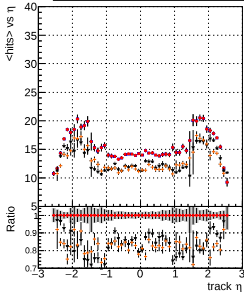
— DQM_XiMinus_original_lowpt — DQM_XiMinus_newbranch_lowpt — DQM_XiMinus_original_lowpt_pLess — DQM_XiMinus_newbranch_lowpt_pLess mean hits
