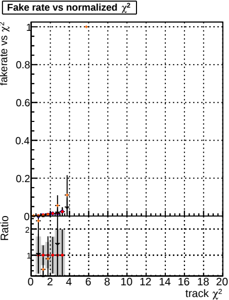
Fake rate vs. original lowpt original lowpt pLess newbranch lowpt pLess
