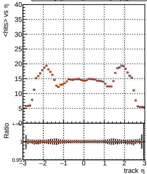
Legend: — DQM_XiMinus_original_lowpt — DQM_XiMinus_newbranch_lowpt — DQM_XiMinus_original_lowpt_pLess — DQM_XiMinus_newbranch_lowpt_pLess
