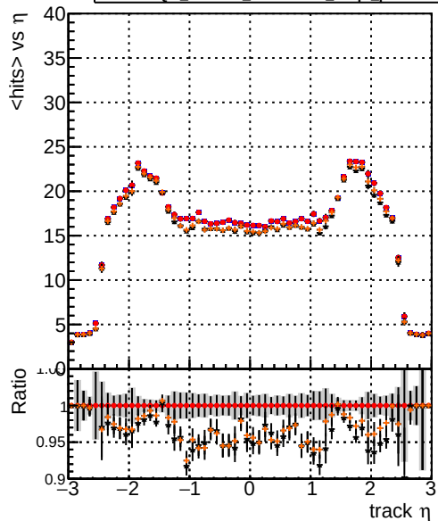
Legend: — DQM_XiMinus_original_lowpt (blue line) — DQM_XiMinus_newbranch_lowpt (red line) — DQM_XiMinus_original_lowpt_pLess (black line) — DQM_XiMinus_newbranch_lowpt_pLess (orange line) mean hits
