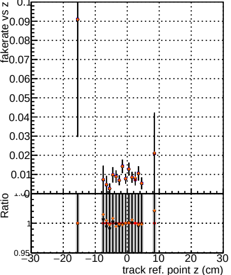
Fake rate vs v Legend: DOM XMinus original lowpt DOM XMinus newbranch lowpt DOM XMinus original lowpt pLess DOM XMinus newbranch lowpt pLess
