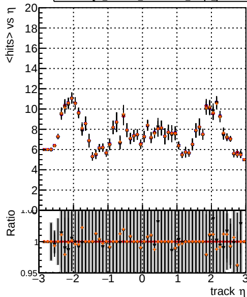
mean hits vs \eta — DQM_XiMinus_original_lowpT — DQM_XiMinus_newbranch_lowpT — DQM_XiMinus_original_lowpT_pLess — DQM_XiMinus_newbranch_lowpT_pLess
