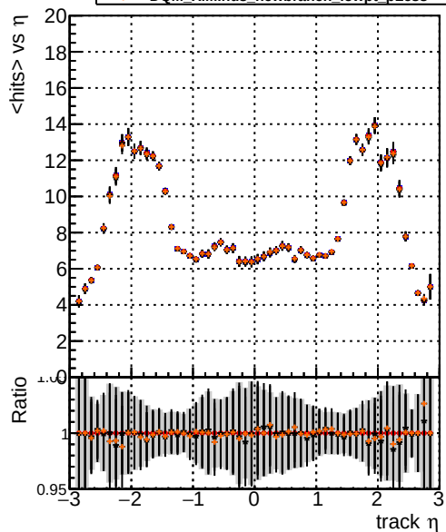
Legend: — DQM_XiMinus_original_lowpt (blue line) — DQM_XiMinus_newbranch_lowpt (red line) — DQM_XiMinus_original_lowpt_pLess (black line) — DQM_XiMinus_newbranch_lowpt_pLess (orange line)
