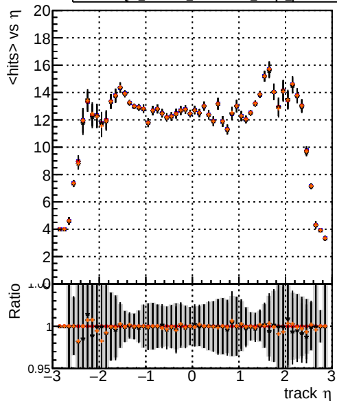
mean hit Legend: - DQM_XiMinus_original_lowpt (blue line) - DQM_XiMinus_newbranch_lowpt (red line with dots) - DQM_XiMinus_original_lowpt_pLess (black line with dots) - DQM_XiMinus_newbranch_lowpt_pLess (orange line with dots)
