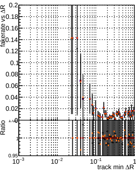
Fake rate vs \Delta R(\text{track}, \text{jet}) Legend: DOM (black line) XiMinus (blue line) original lowpt (red line) newbranch lowpt (orange line) original lowpt pLess (black line) newbranch lowpt pLess (orange line)
