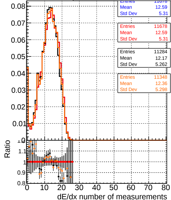
—●— DQM_XiMinus_original_lowpt —●— DQM_XiMinus_newbranch_lowpt —●— DQM_XiMinus_original_lowpt_pLess —●— DQM_XiMinus_newbranch_lowpt_pLess
