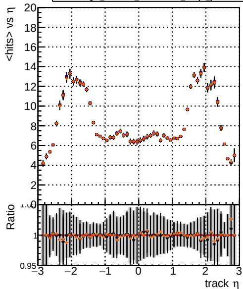
— DQM_XiMinus_original_lowpt — DQM_XiMinus_newbranch_lowpt — DQM_XiMinus_original_lowpt_pLess — DQM_XiMinus_newbranch_lowpt_pLess mean hit
