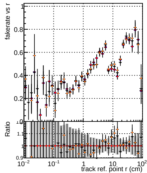
DOM X Minus original lowpt DOM X Minus newbranch lowpt DOM X Minus original lowpt pLess DOM X Minus newbranch lowpt pLess
