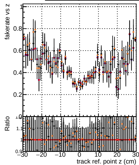
DOM X Minus original lowpt DOM X Minus newbranch lowpt DOM X Minus original lowpt pLess DOM X Minus newbranch lowpt pLess
