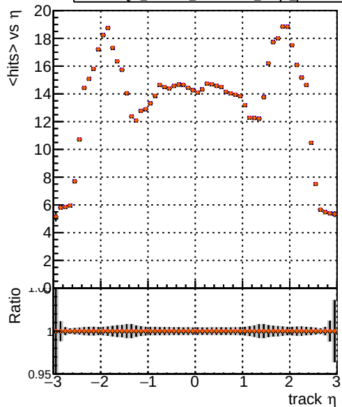
mean hits vs \eta DQM_XiMinus_original_lowpt DQM_XiMinus_newbranch_lowpt DQM_XiMinus_original_lowpt_pLess DQM_XiMinus_newbranch_lowpt_pLess
