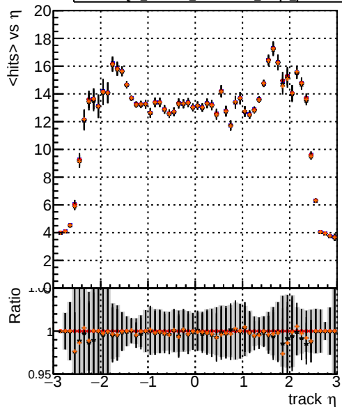
mean hits Legend: DQM_XiMinus_original_lowpt (blue line), DQM_XiMinus_newbranch_lowpt (red line), DQM_XiMinus_original_lowpt_pLess (black line), DQM_XiMinus_newbranch_lowpt_pLess (orange line)
