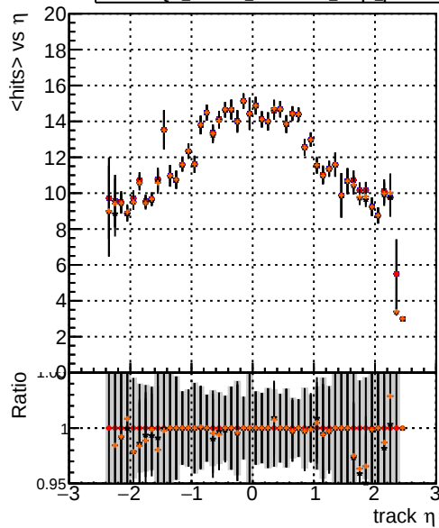
Legend: — DQM_XiMinus_original_lowpt (blue line) — DQM_XiMinus_newbranch_lowpt (red line) — DQM_XiMinus_original_lowpt_pLess (black line) — DQM_XiMinus_newbranch_lowpt_pLess (orange line) mean hit
