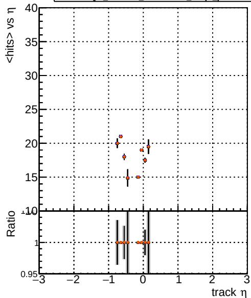
mean hit DQM_XiMinus_original_lowpt DQM_XiMinus_newbranch_lowpt DQM_XiMinus_original_lowpt_pLess DQM_XiMinus_newbranch_lowpt_pLess
