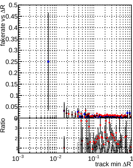
Fake rate vs ΔR(track, jet) Legend: DQM XiMinus original (blue dots) DQM XiMinus newbranch pLess (red dots) DQM XiMinus newbranch pLessMVACand (black dots)
