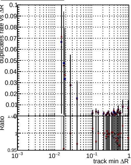
Legend: DQM XiMinus original (black line with blue dots), DQM XiMinus newbranch (black line with red dots), DQM XiMinus newbranch pLess (black line with black dots)
