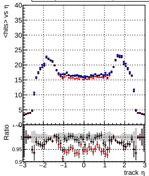
mean hits vs \eta DQM_XiMinus_original DQM_XiMinus_newbranch_pLess DQM_XiMinus_newbranch_pLessMVACand
