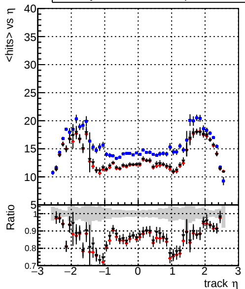
mean hits — DQM_XiMinus_original — DQM_XiMinus_newbranch_pLess — DQM_XiMinus_newbranch_pLessMVACand
