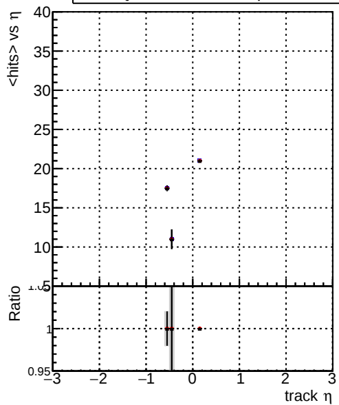
mean hit — DQM_XiMinus_original — DQM_XiMinus_newbranch_pLess — DQM_XiMinus_newbranch_pLessMVACand
