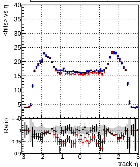
mean hit — DQM_XiMinus_original — DQM_XiMinus_newbranch_pLess — DQM_XiMinus_newbranch_pLessMVACand
