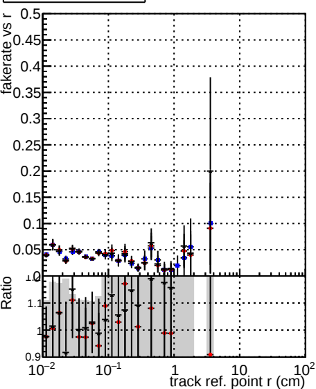
Fake rate vs vertpos —●— DQM_XiMinus_original —●— DQM_XiMinus_newbranch_pLess —●— DQM_XiMinus_newbranch_pLessMVACand
