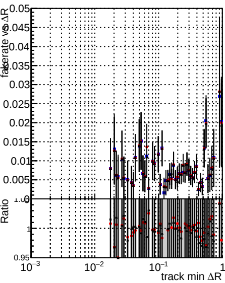
DOM_XiMinus_original DOM_XiMinus_newbranch_pLess DOM_XiMinus_newbranch_pLessMVACand
