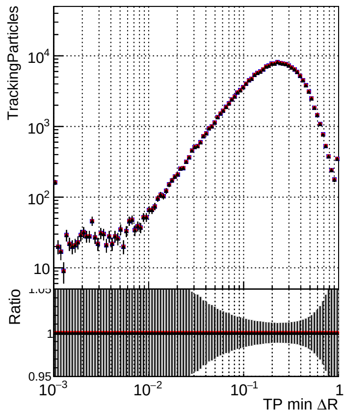
N of simulated tracks vs TP \Delta R (TP, jet) DQM_XiMinus_original DQM_XiMinus_newbranch_pLess DQM_XiMinus_newbranch_pLessMVA Cand
