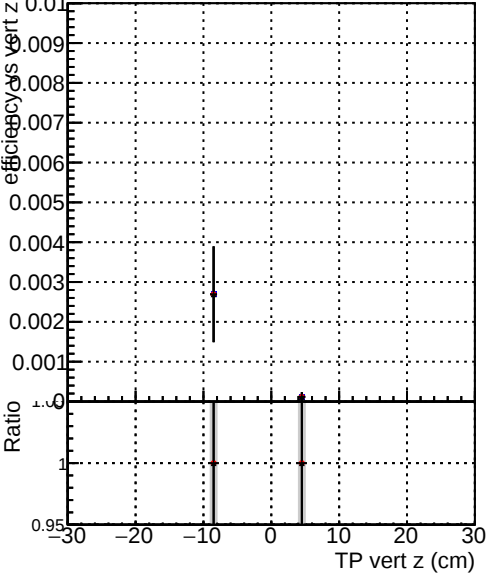
Efficiency vs TP vert z Legend: DQM_XiMinus_original (blue line with circles) DQM_XiMinus_newbranch_pLess (red line with circles) DQM_XiMinus_newbranch_pLessMVACand (black line with circles)
