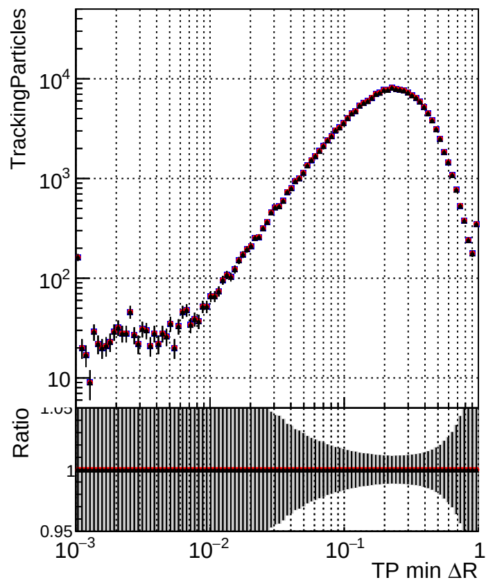
N of simulated tracks vs TP \Delta R (TP, jet) DQM_XiMinus_original DQM_XiMinus_newbranch_pLess DQM_XiMinus_newbranch_pLessMVAand
